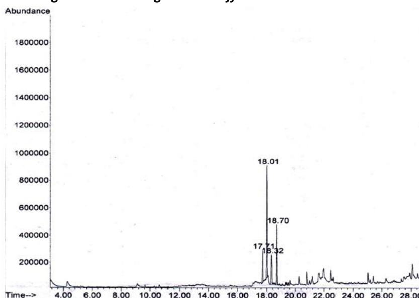
Figure 1 Chromatogram of Z. officinale ethanolic extract
